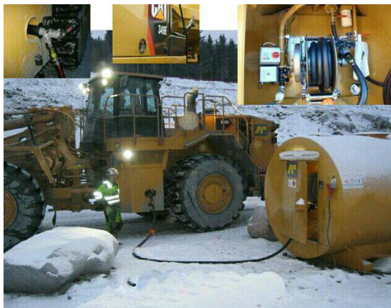
Automatic Nozzle
